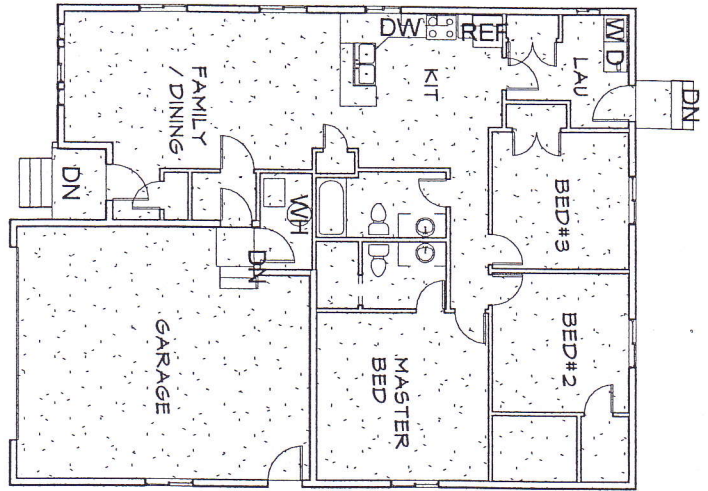
1 SPEC PLAN 1/16" = 1'-0" 1450 SQ.FT.
